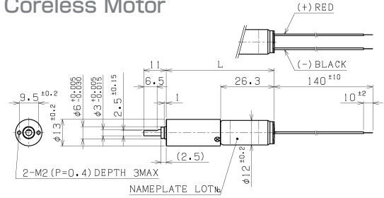
*THE CABLE LOCATION IS FOR REFERENCE ONLY. Unit : mm
